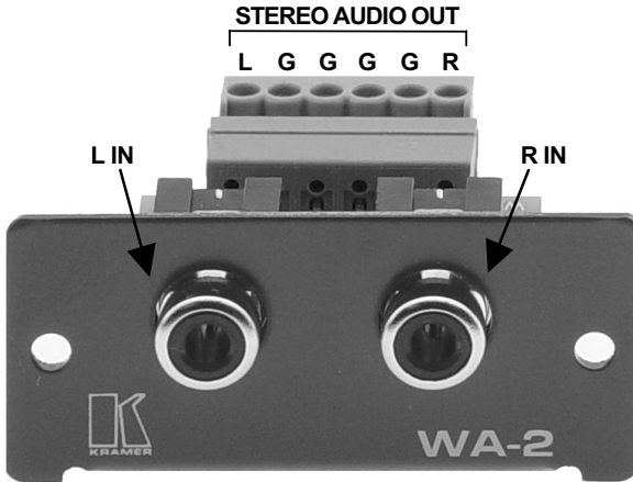
Figure 3: WA-2 Dual RCA to Terminal Block Adapter
