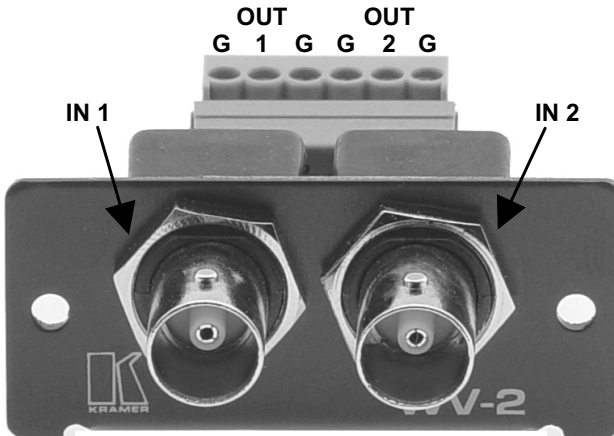
Figure 4: WV-2 Dual BNC to Terminal Block Adapter
